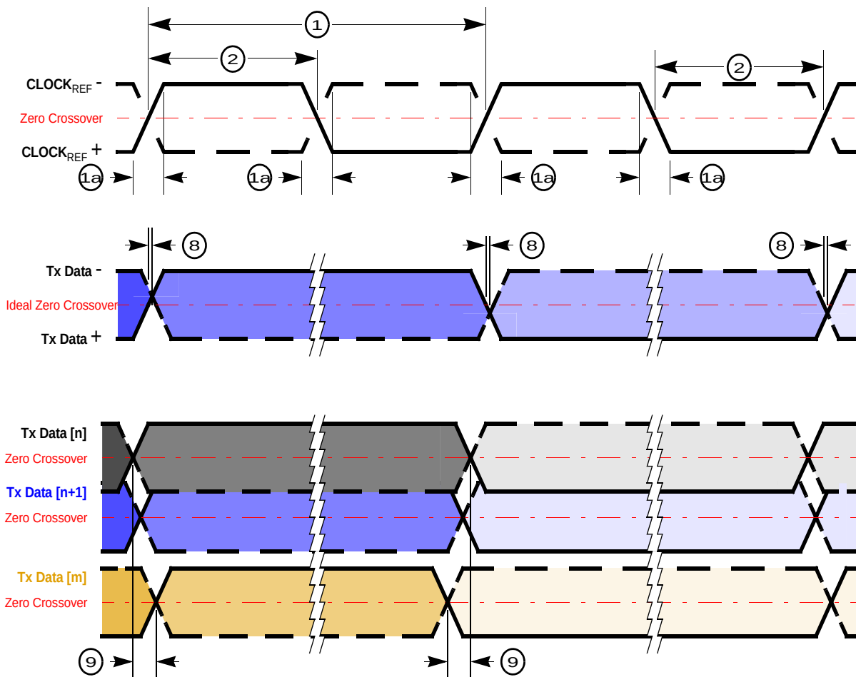
Figure 28. Aurora timings
