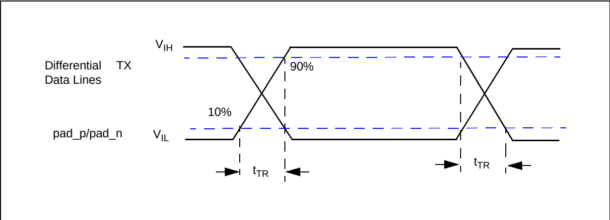
Figure 18. Rise/fall time
