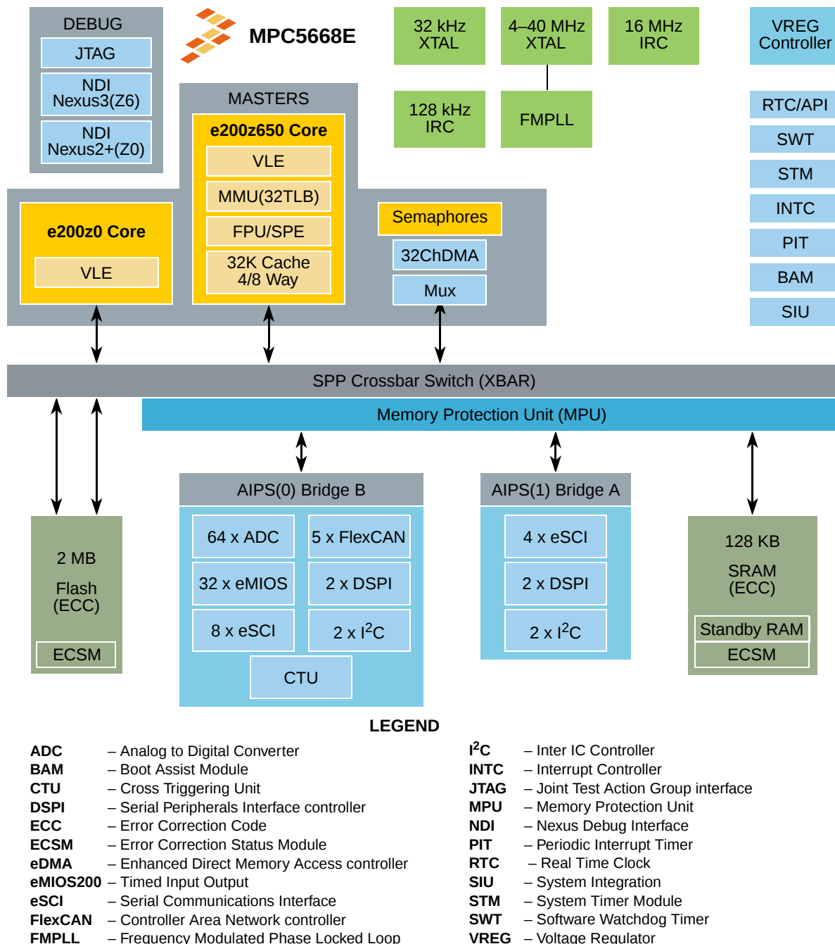
Figure 2. MPC5668E Block Diagram
