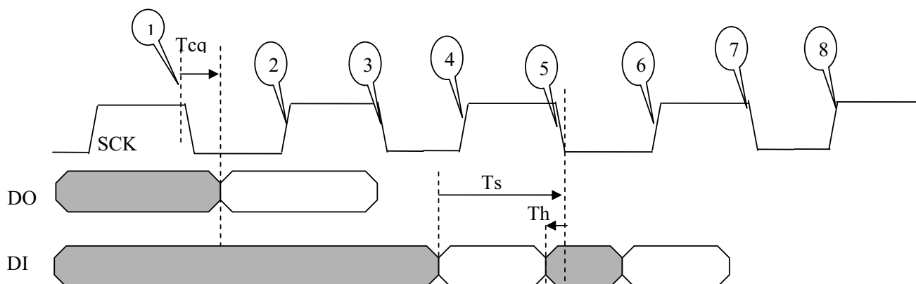
Figure 45. QuadSPI output timing
