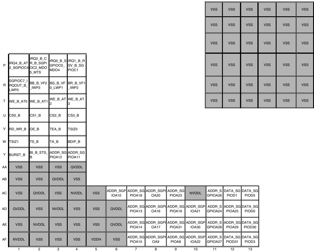
Figure G-67. MPC561/MPC563 Ball Map (Black and White, page 2)
