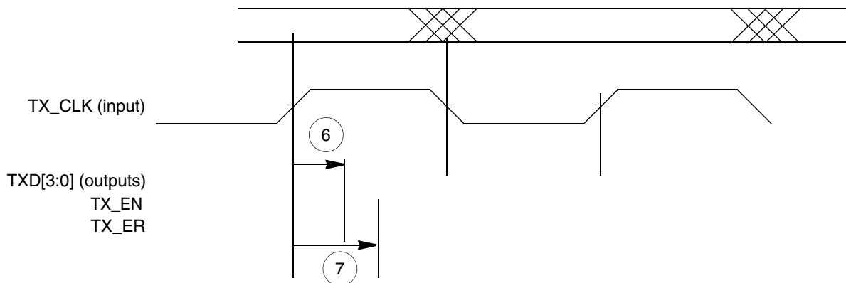
Figure 35. MII transmit signal timing diagram
