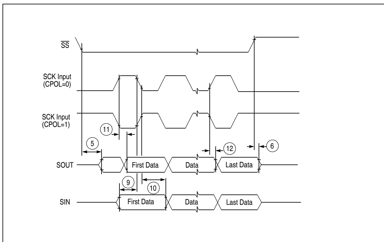
Figure 31. DSPI modified transfer format timing — Slave, CPHA = 1
