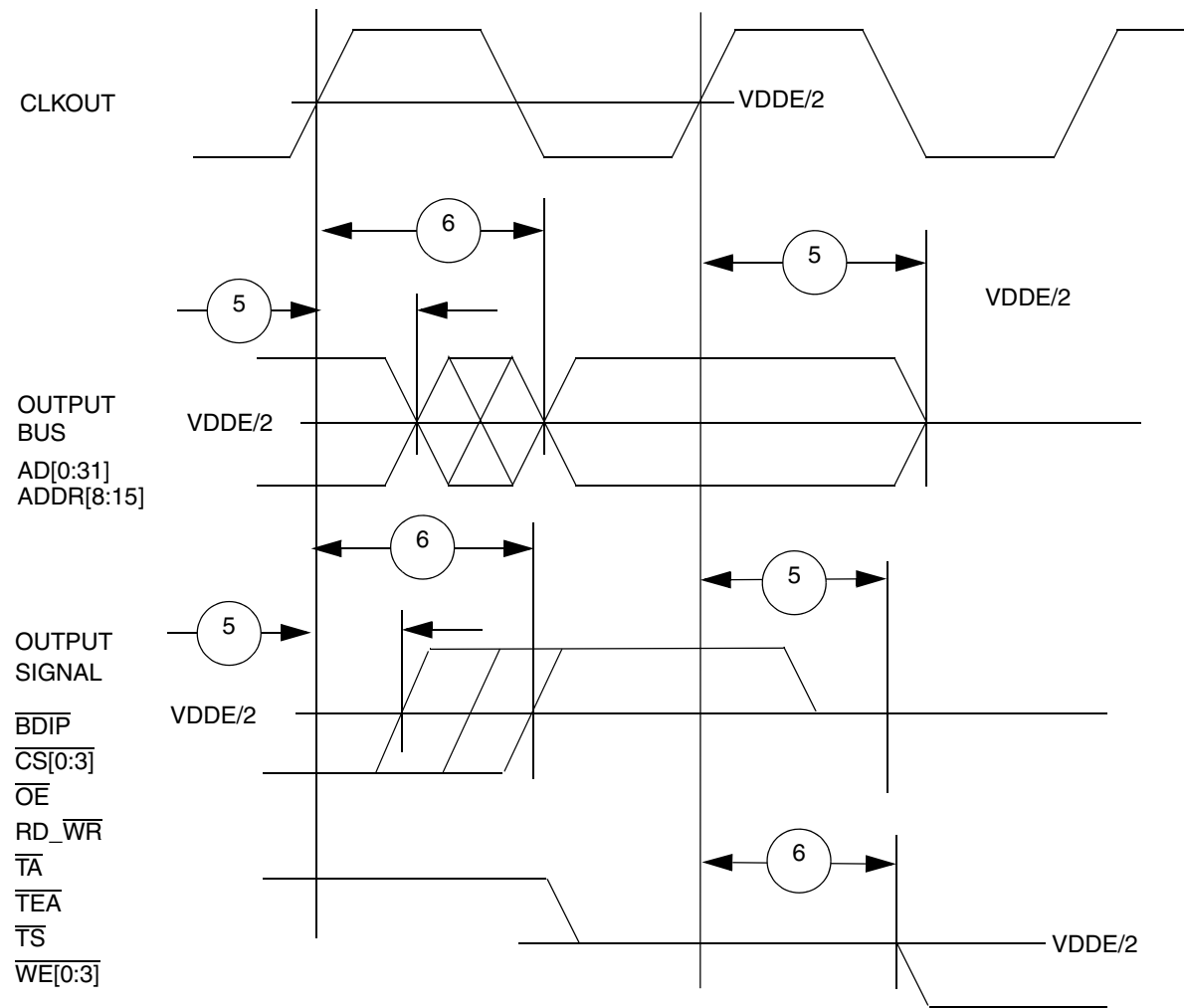
Figure 15. Synchronous Output Timing
