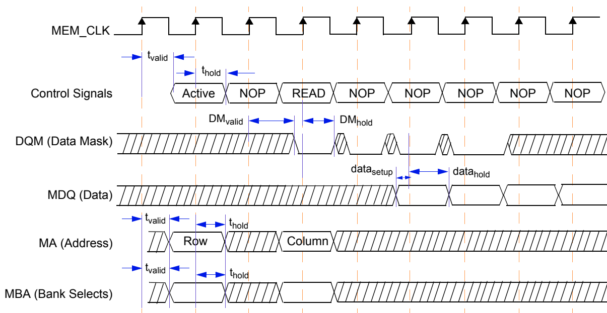
Figure 5. Timing Diagram—Standard SDRAM Memory Read Timing
