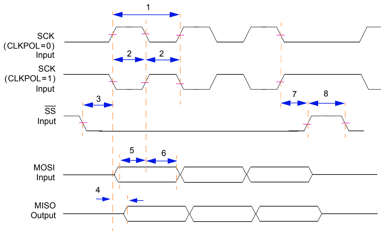
Figure 36. Timing Diagram — SPI Slave Mode, Format 1 (CPHA = 1)
