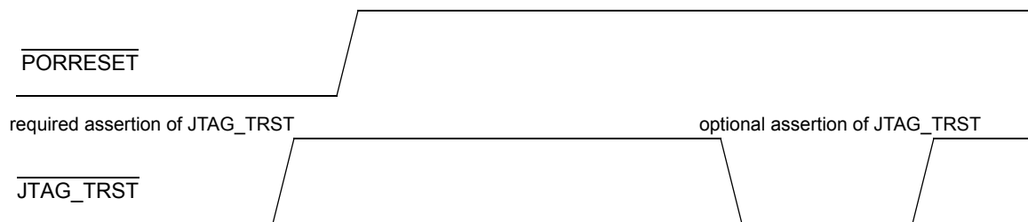
Figure 54. PORRESET vs. JTAG_TRST
