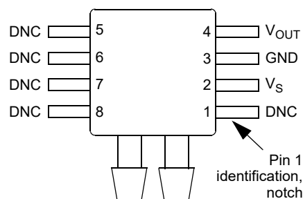
Pinout
