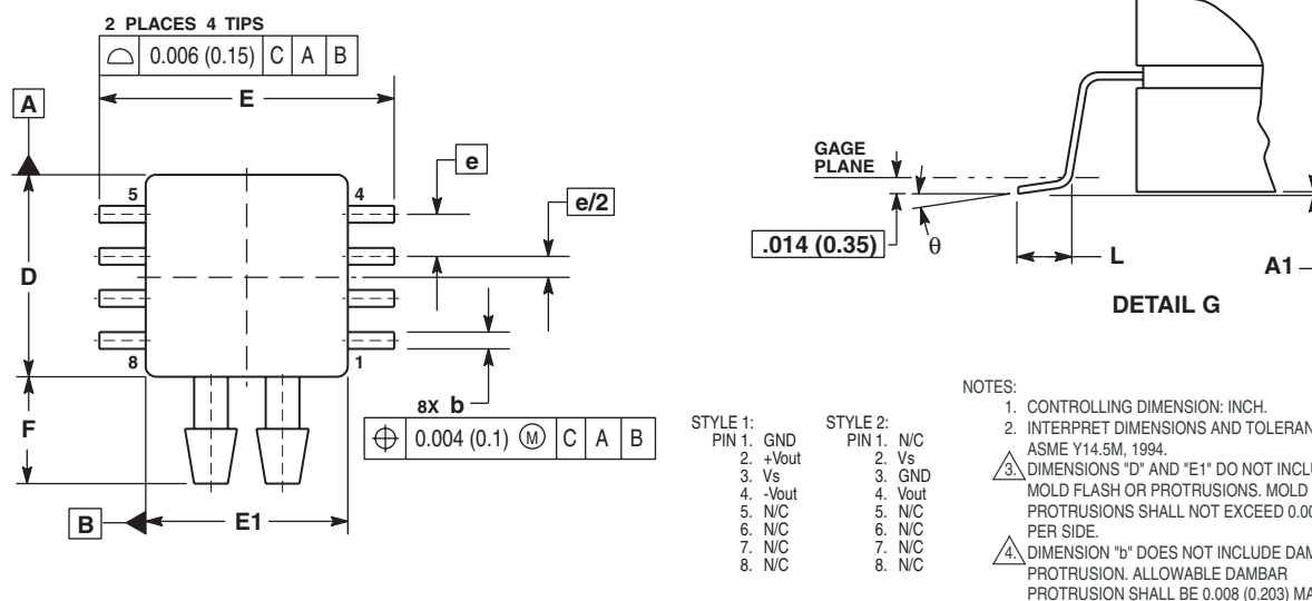
CASE 482A-01 ISSUE A SMALL OUTLINE PACKAGE
