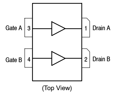
Figure 1. Pin Connections
