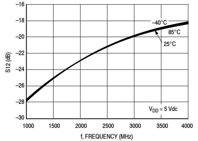
Figure 5. S12 versus Frequency and Temperature
