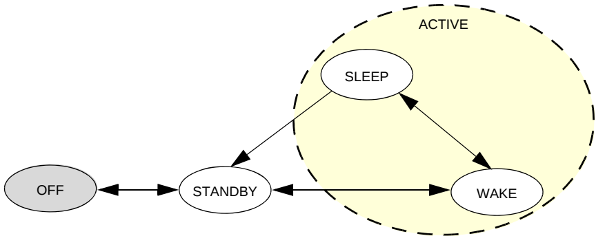
Figure 5. Operating modes for MMA8653FC
