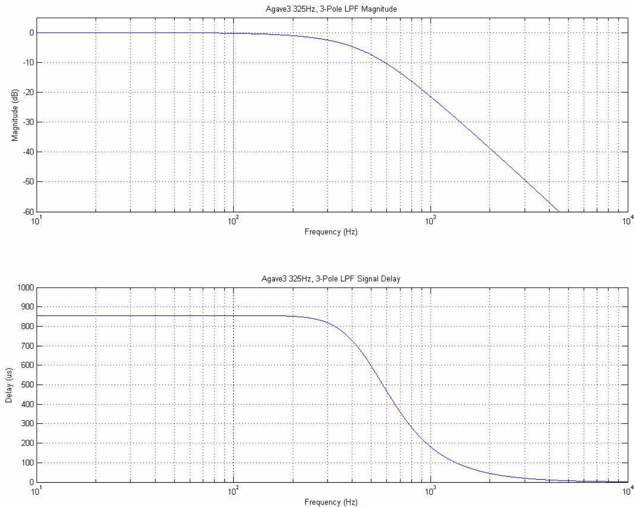
Figure 18. Low-pass filter characteristics: f_C = 325 \text{ Hz} , 3-Pole, t_S = 16 \mu\text{s}
