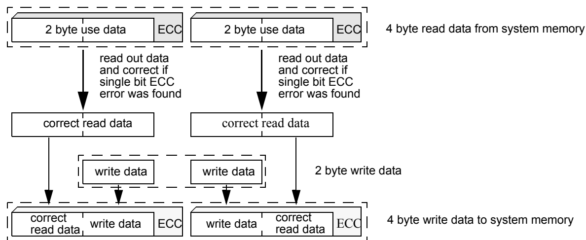
Figure 63. 2 Byte non-aligned write access
