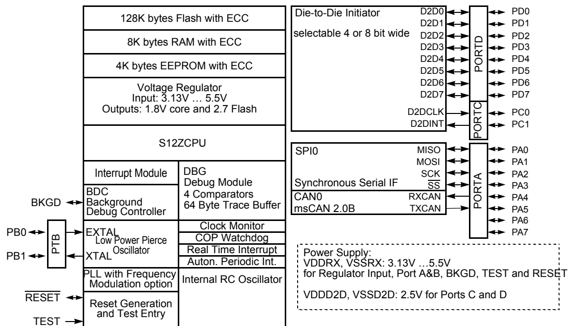
Figure 17. MC9S12ZI128 block diagram
