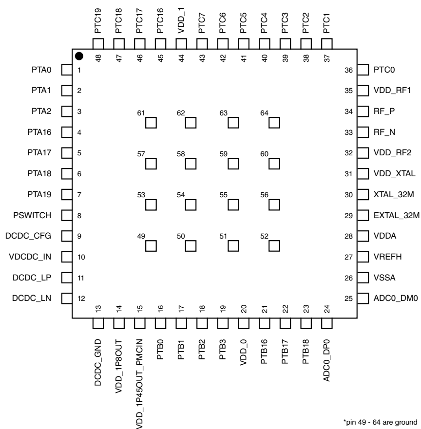
Figure 17. 48-pin Laminate QFN pinout diagram
