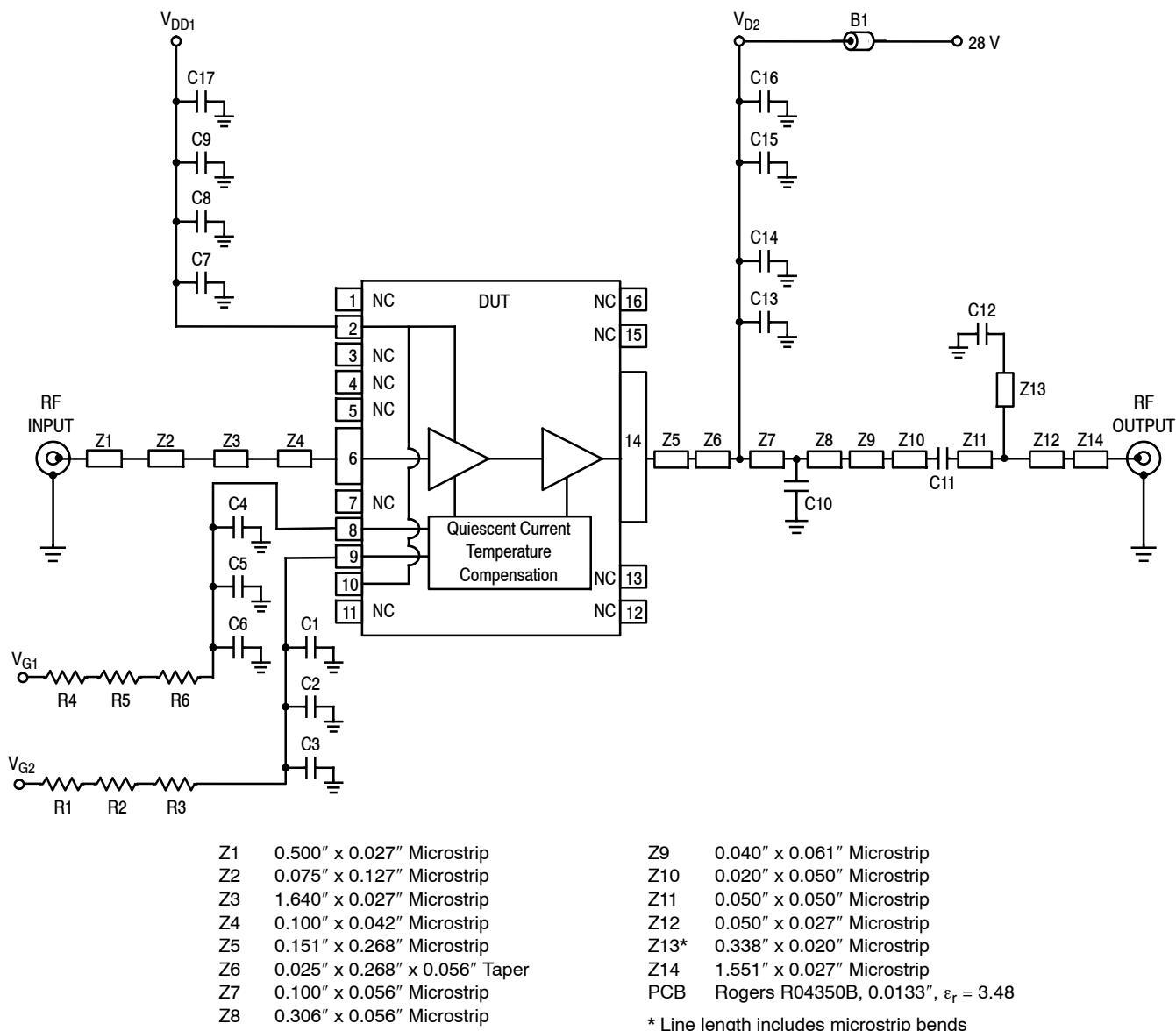
Figure 3. MHT2000NR1 Narrowband Test Circuit Schematic
