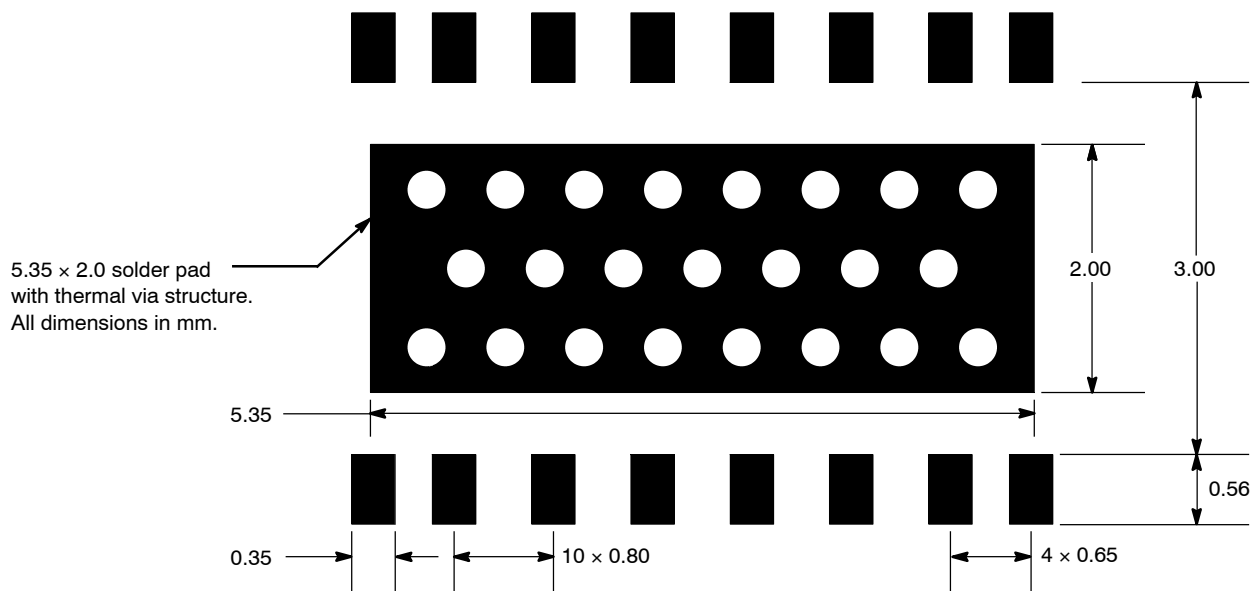
Figure 11. PCB Pad Layout for 16-Lead DFN 4 x 6
