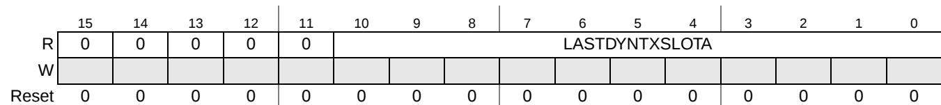
Figure 3-59. Last Dynamic Slot Channel A Register (LDTXSLAR)
