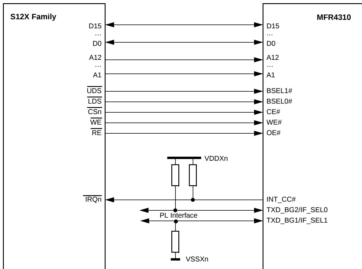
Figure 2-5. AMI Interface with S12X Family
