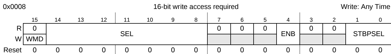
Figure 3-4. Strobe Signal Control Register (STBSCR)
