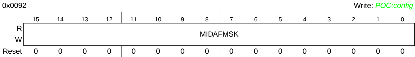
Figure 3-54. Receive FIFO Message ID Acceptance Filter Mask Register (RFMIAFMR)
