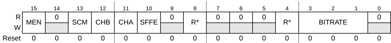
Figure 3-3. Module Configuration Register (MCR)
