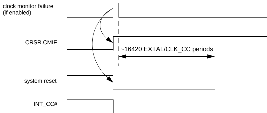
Figure 6-5. Clock Monitor Failure Reset
