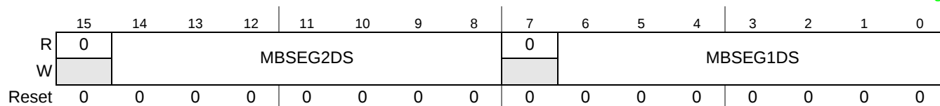
Figure 3-5. Message Buffer Data Size Register (MBDSR)
