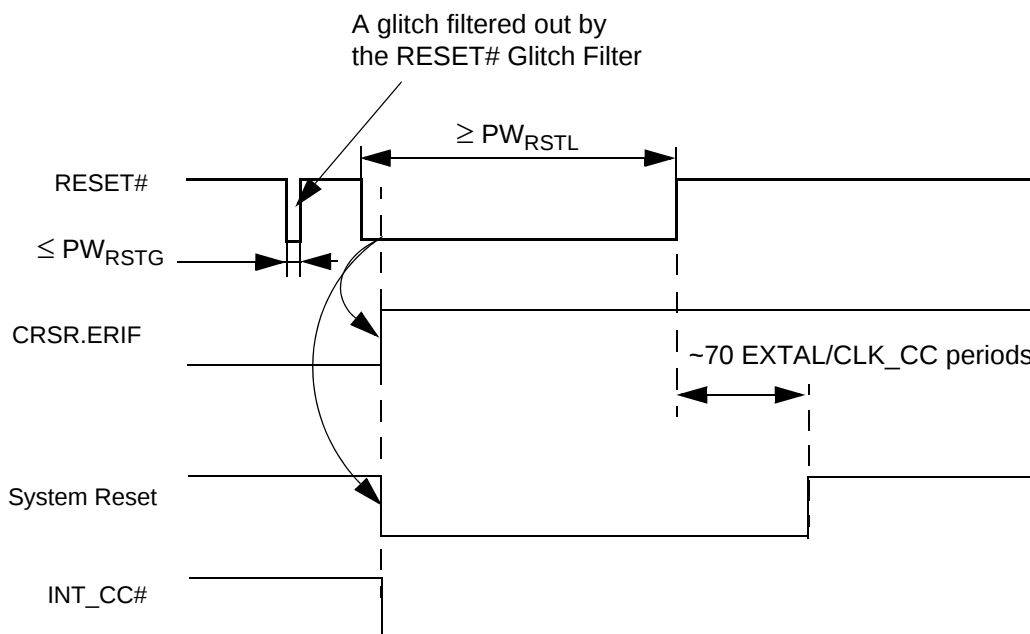
Figure 6-6. External Reset
