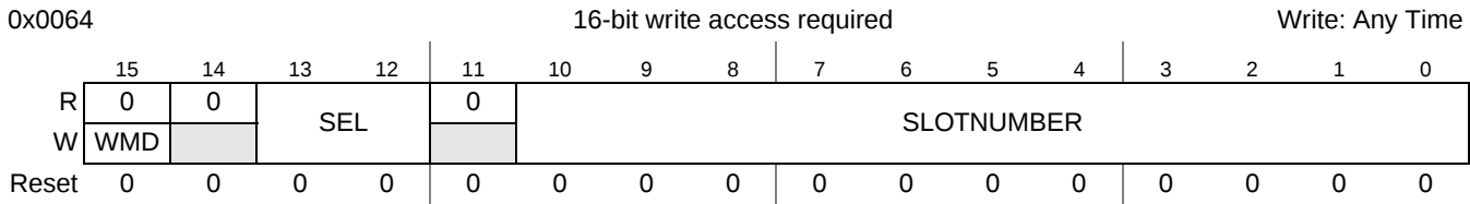
Figure 3-41. Slot Status Selection Register (SSSR)
