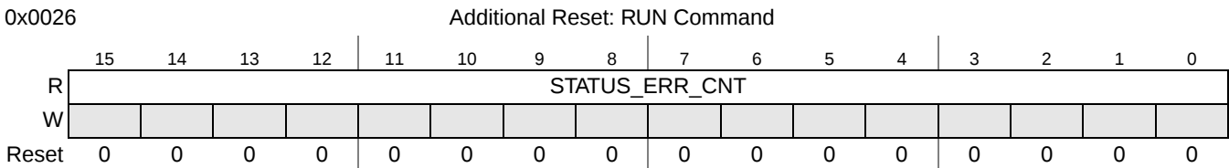
Figure 3-16. Channel B Status Error Counter Register (CBSECR)
