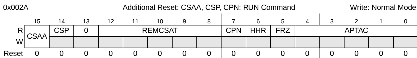
Figure 3-18. Protocol Status Register 1 (PSR1)
