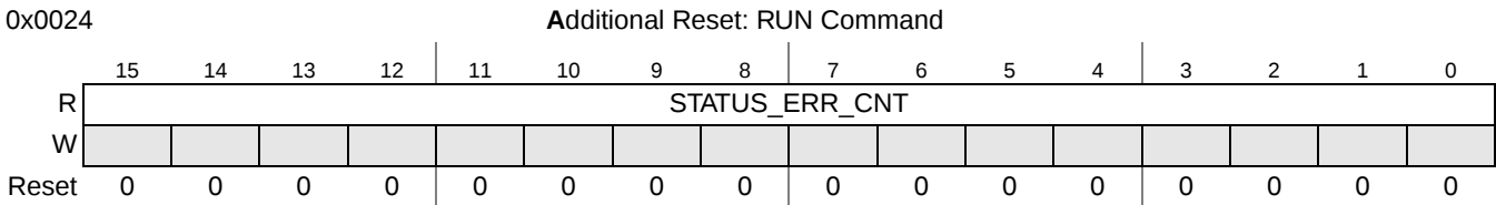
Figure 3-15. Channel A Status Error Counter Register (CASERCR)
