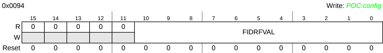
Figure 3-55. Receive FIFO Frame ID Rejection Filter Value Register (RFFIDRFVR)
