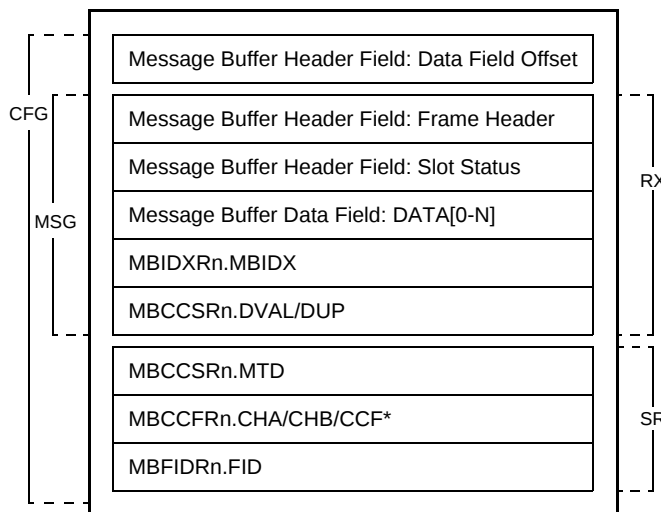
Figure 3-117. Receive Message Buffer Access Regions
