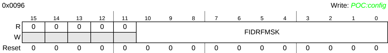
Figure 3-56. Receive FIFO Frame ID Rejection Filter Mask Register (RFFIDRFMR)
