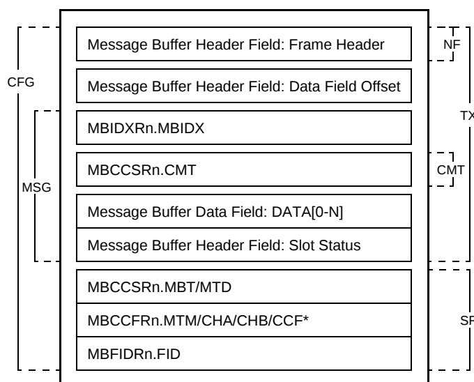
Figure 3-109. Single Transmit Message Buffer Access Regions
