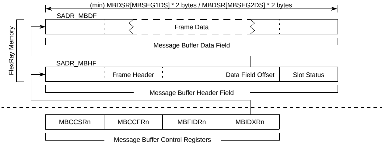
Figure 3-97. Individual Message Buffer Structure
