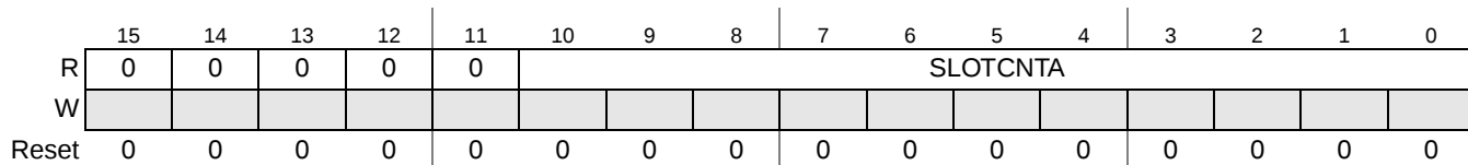
Figure 3-23. Slot Counter Channel A Register (SLTCTAR)
