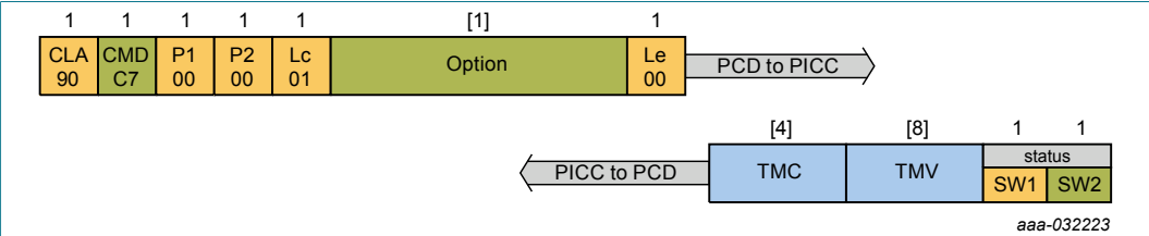
Figure 38. CommitTransaction command protocol
