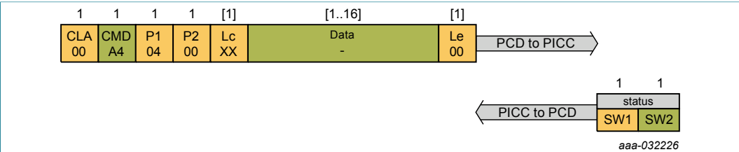
Figure 41. ISOSelectFile command protocol
