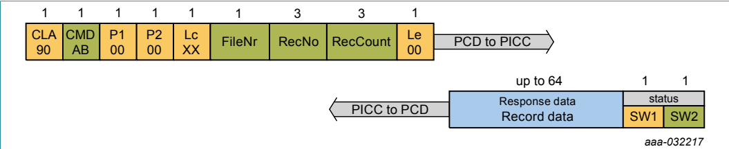
Figure 34. ReadRecords command protocol
