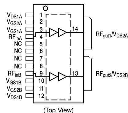
Figure 2. Pin Connections
