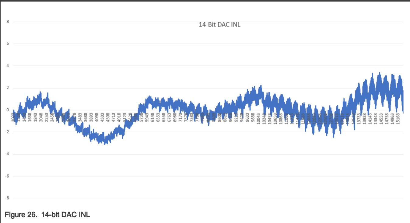
Figure 26. 14-bit DAC INL
