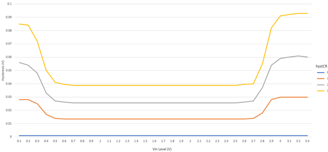
Figure 29. Typical hysteresis vs. Vin level (VDD = 3.3 V, HPMD = 0, NPMD = 1)
