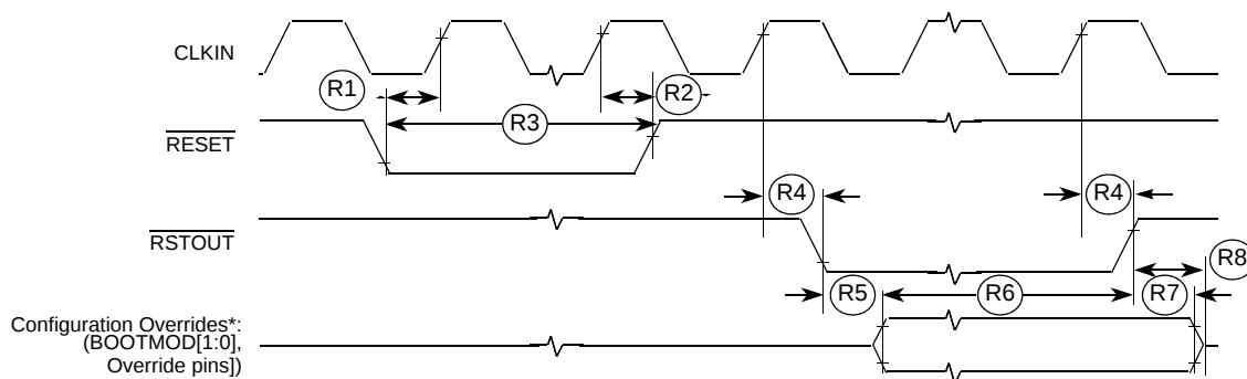
Figure 8. RESET and Configuration Override Timing
