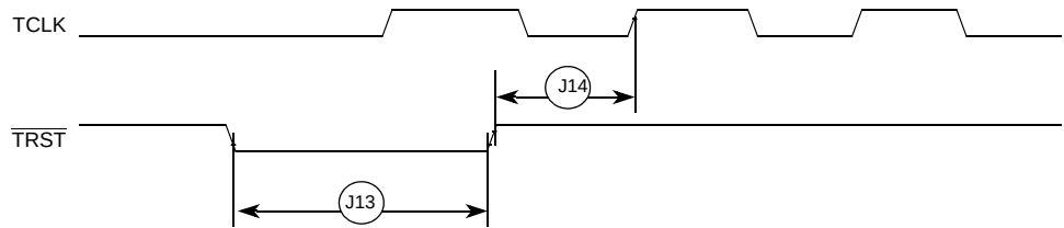
Figure 31. \overline{\text{TRST}} Timing
