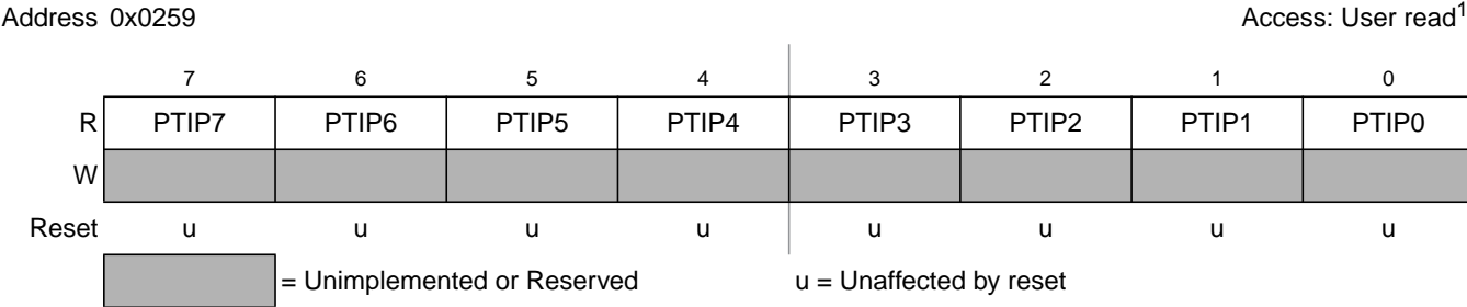
Figure 2-41. Port P Input Register (PTIP)
