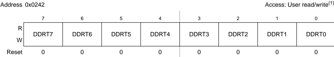
Figure 19-21. Port T Data Direction Register (DDRT)
