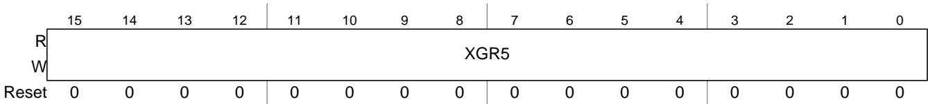
Figure 14-19. XGATE Register 5 (XGR5)
