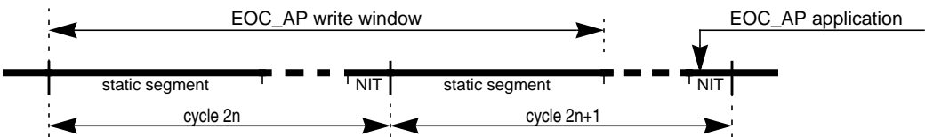
Figure 13-136. External Offset Correction Write and Application Timing
