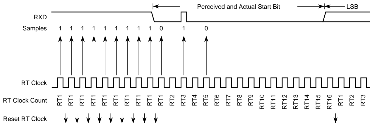
Figure 23-25. Start Bit Search Example 4
