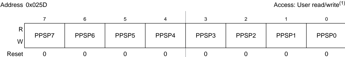
Figure 19-48. Port P Polarity Select Register (PPSP)
