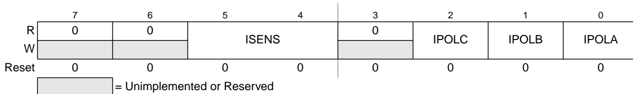
Figure 20-19. PMF Correction Control Register (PMFCCTL)
