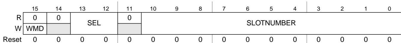
Figure 13-45. Slot Status Selection Register (SSSR)
