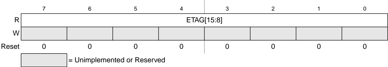
Figure 8-18. EEE Tag Counter High Register (ETAGHI)
