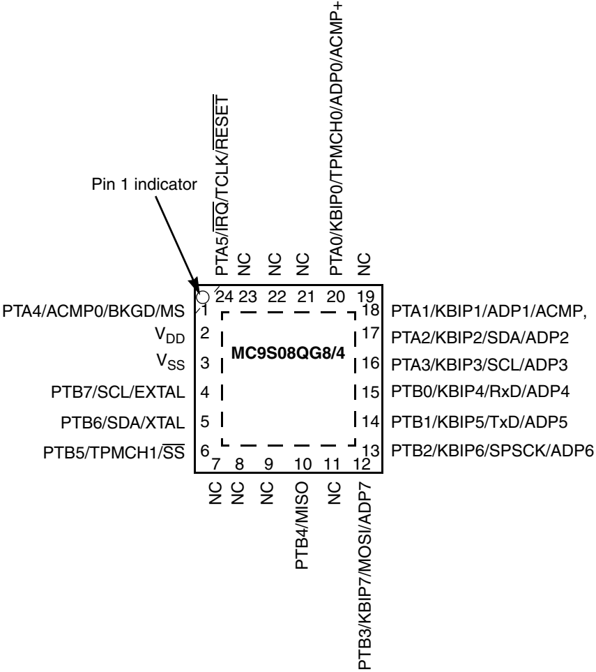
Figure 2-3. 24-Pin Packages
