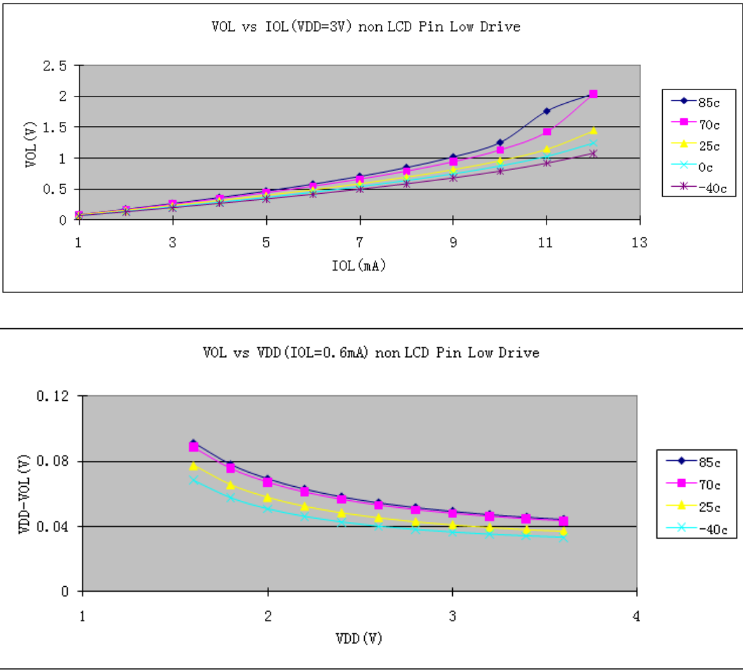
Figure 6. Typical Low-Side Driver (Sink) Characteristics(Non LCD pins) — Low Drive (PTxDSn = 0)
