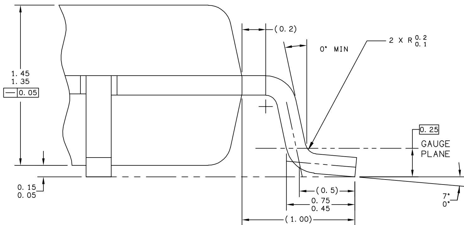
VIEW AA
