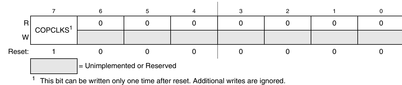
Figure 5-12. System Options Register 2 (SOPT2)
