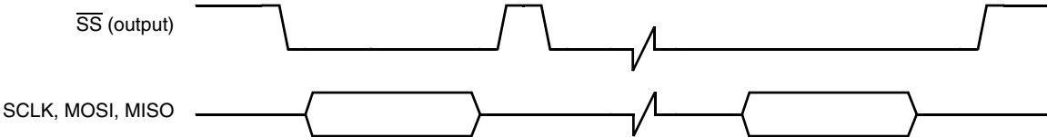
Figure 36. Master SPI Timing Diagram Ignore \overline{\text{SPI\_RDY}} Level Trigger
