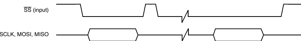
Figure 37. Slave SPI Timing Diagram FIFO Advanced by BIT COUNT
