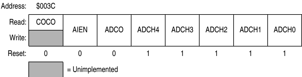
Figure 16-4. ADC Status and Control Register (ADSCR)
