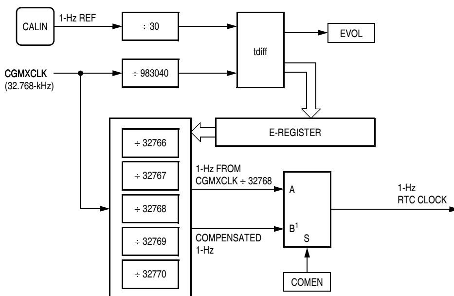
Figure 12-3. RTC Clock Calibration and Compensation
