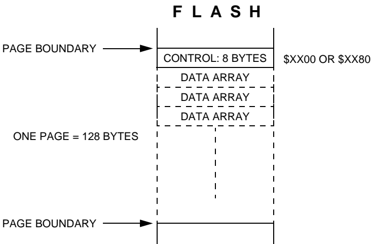
Figure 10-10. EE_WRITE FLASH Memory Usage
