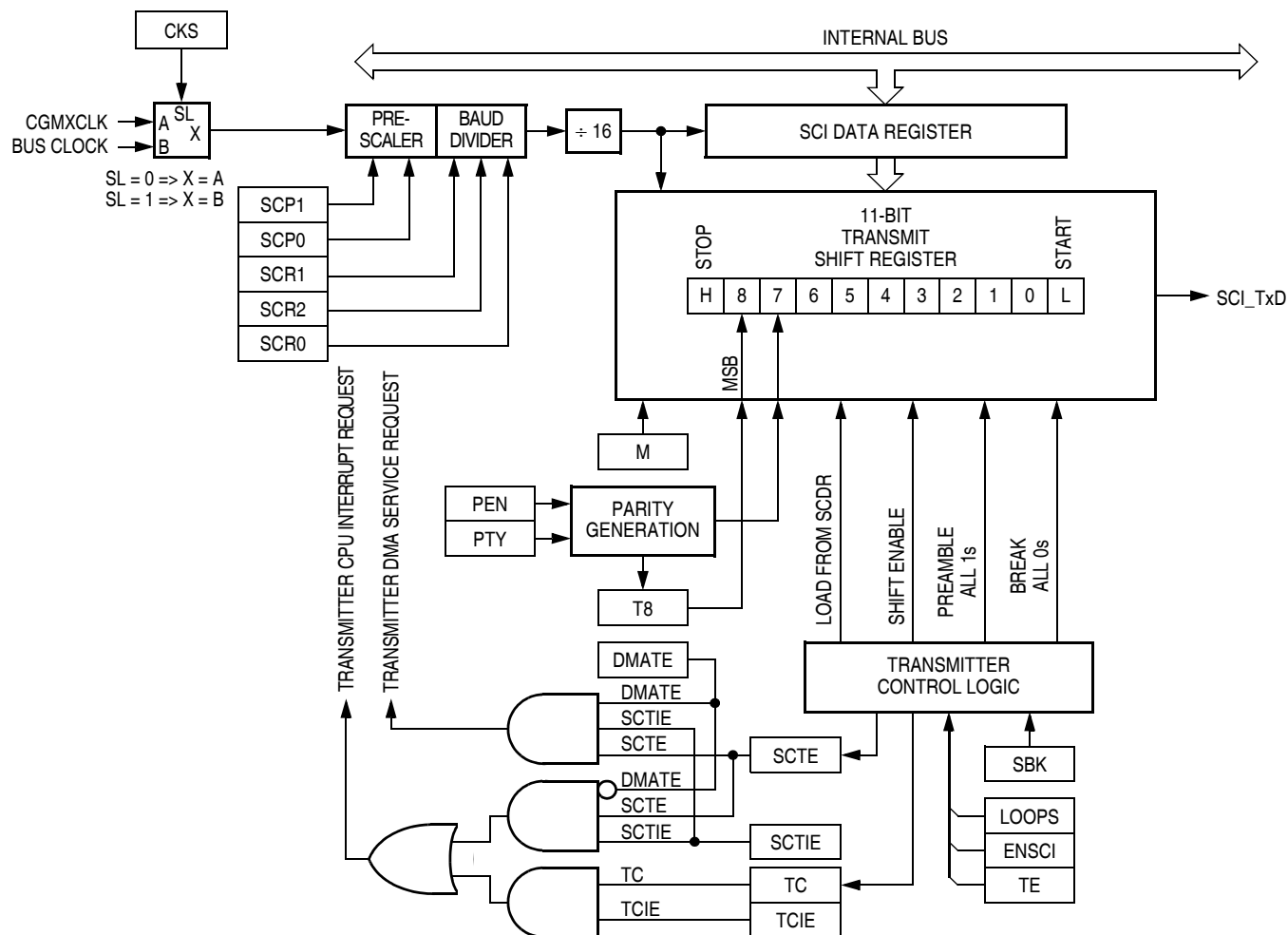
Figure 13-7. SCI Transmitter
