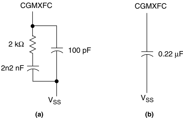
Figure 5-10. PLL Filter
