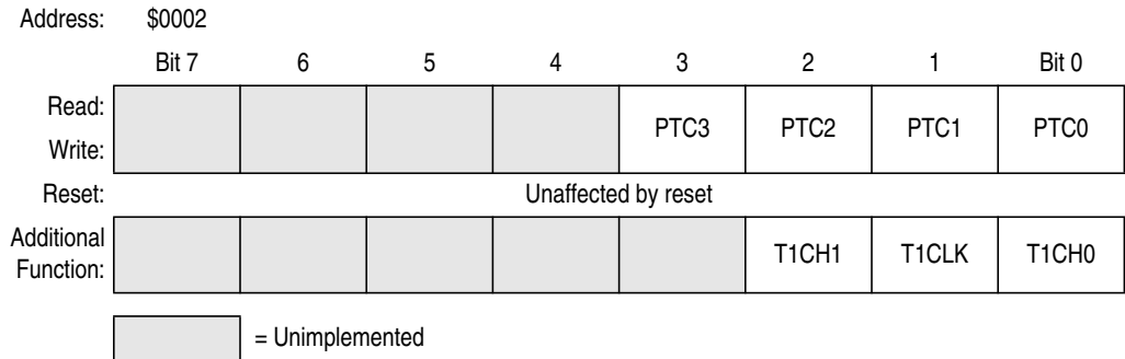
Figure 13-8. Port C Data Register (PTC)
