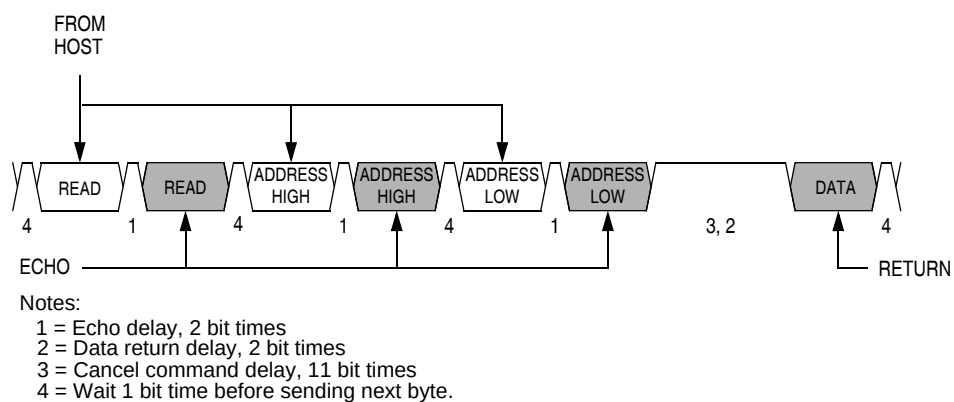
Figure 9-5. Read Transaction
