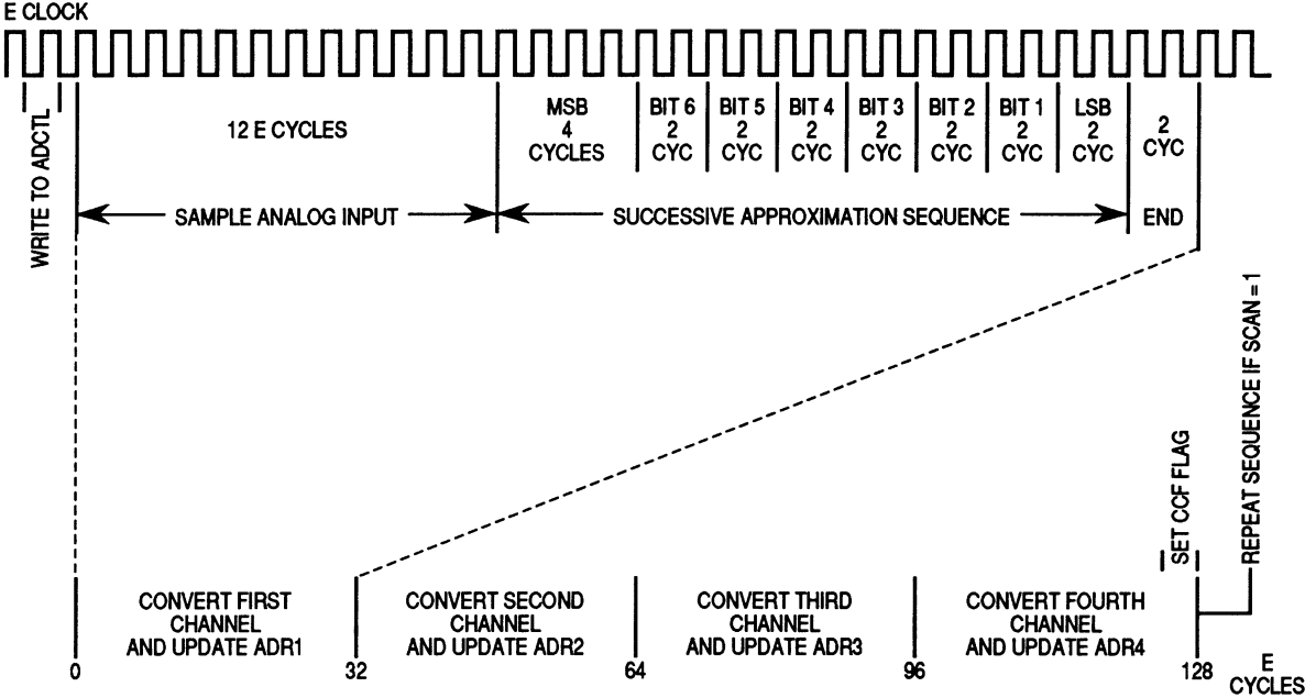
A/D Conversion Sequence
