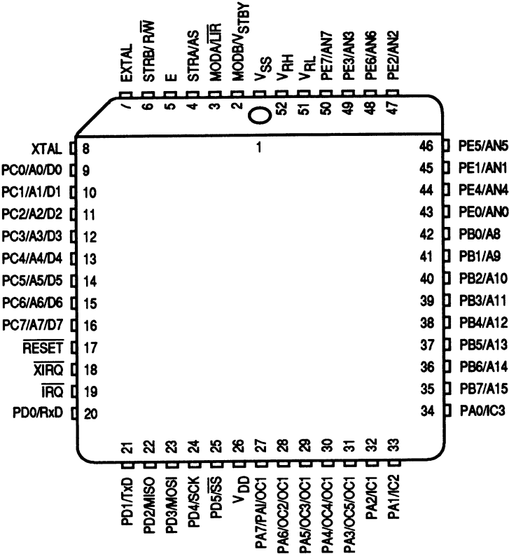
52-Pin PLCC Pin Assignments
