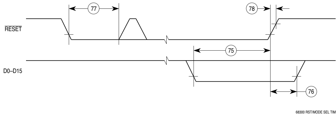
Figure A-12 Reset and Mode Select Timing Diagram
