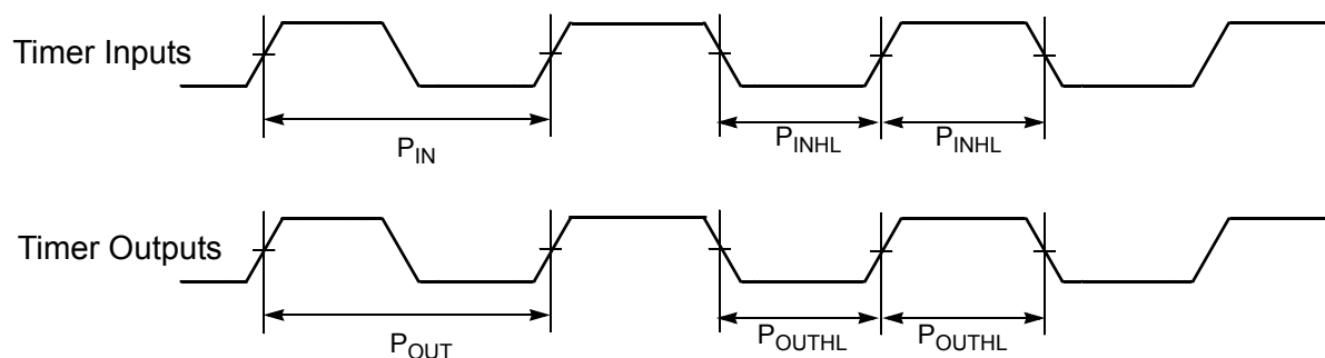
Figure 10-15 Timer Timing
