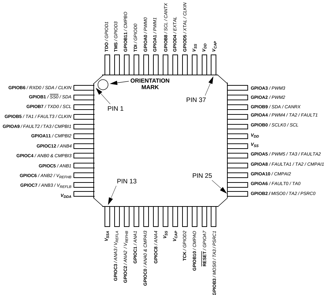
Figure 11-1 Top View, 56F8036 48-Pin LQFP Package
