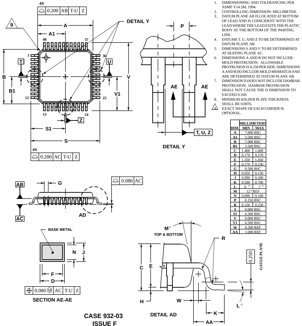
Figure 11-2 56F8036 48-Pin LQFP Mechanical Information
