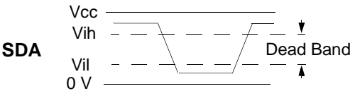
Figure 12. SDA/SCL Levels
