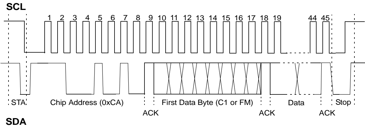
Figure 13. I 2 C Bus Timing
