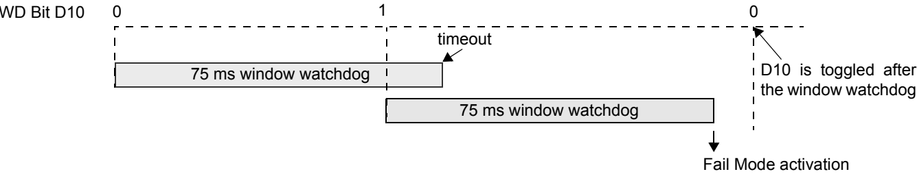
Figure 17. Watchdog window
