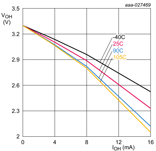
Fig 24. Typical HIGH-level output voltage V_{OH} versus HIGH-level output source current I_{OH}
