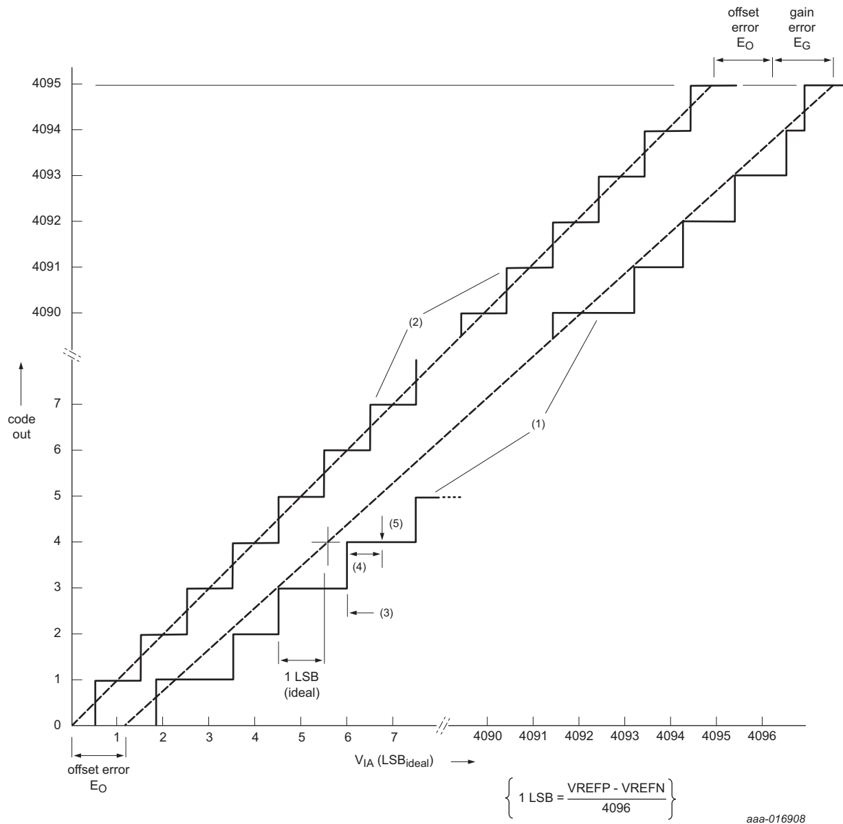
Fig 31. 12-bit ADC characteristics
