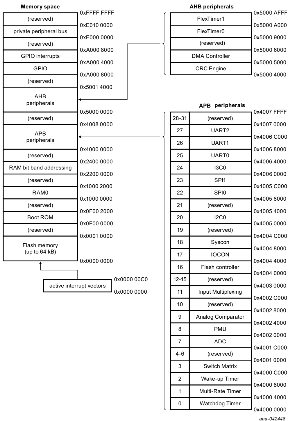
Fig 7. LPC86x AHB Memory mapping
