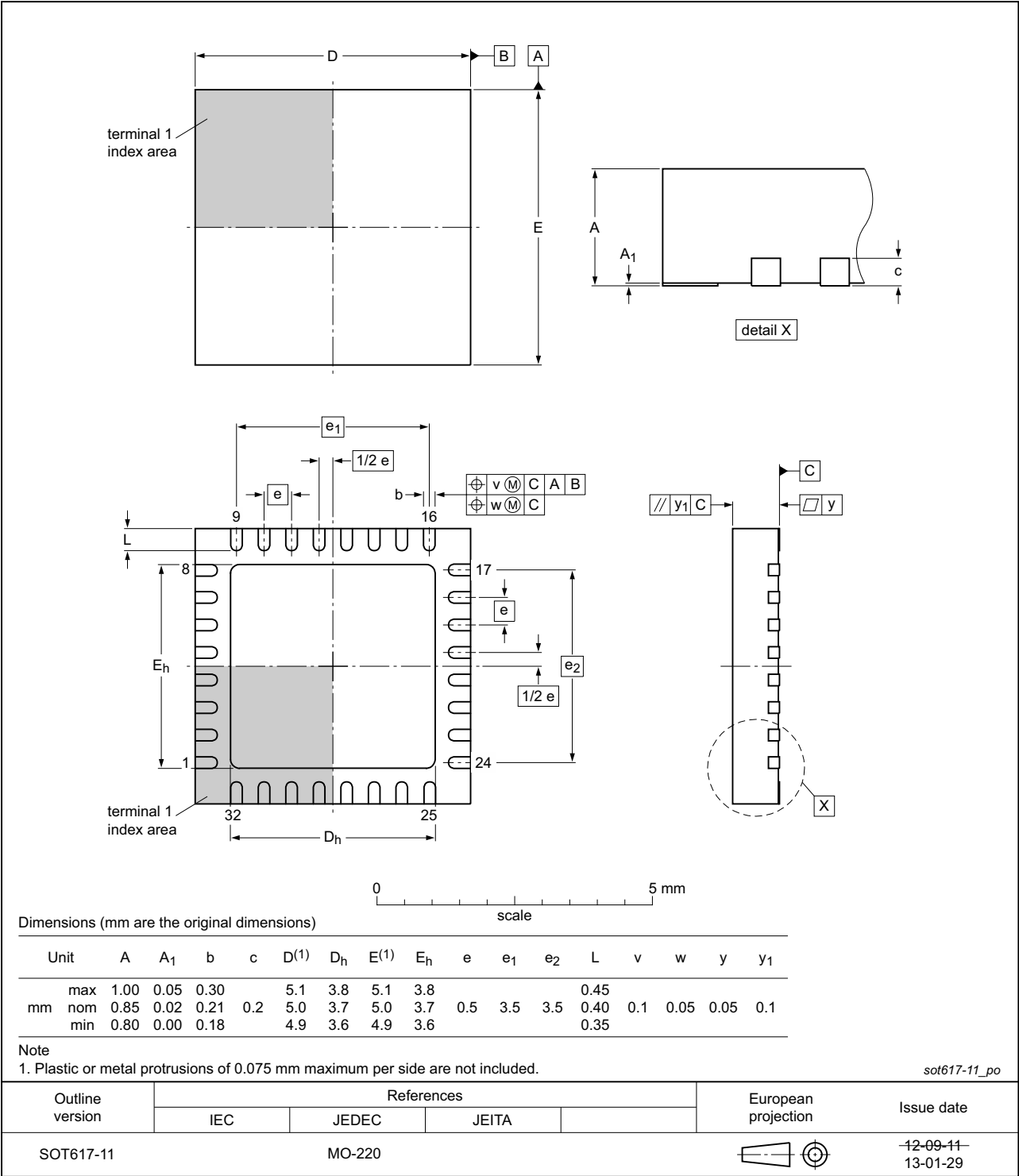
Fig 40. Package outline HVQFN32 5x 5x 0.85 mm (SOT617-11)
