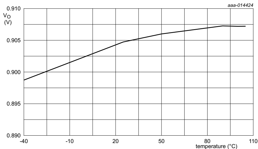
Fig 33. Typical internal voltage reference output voltage
