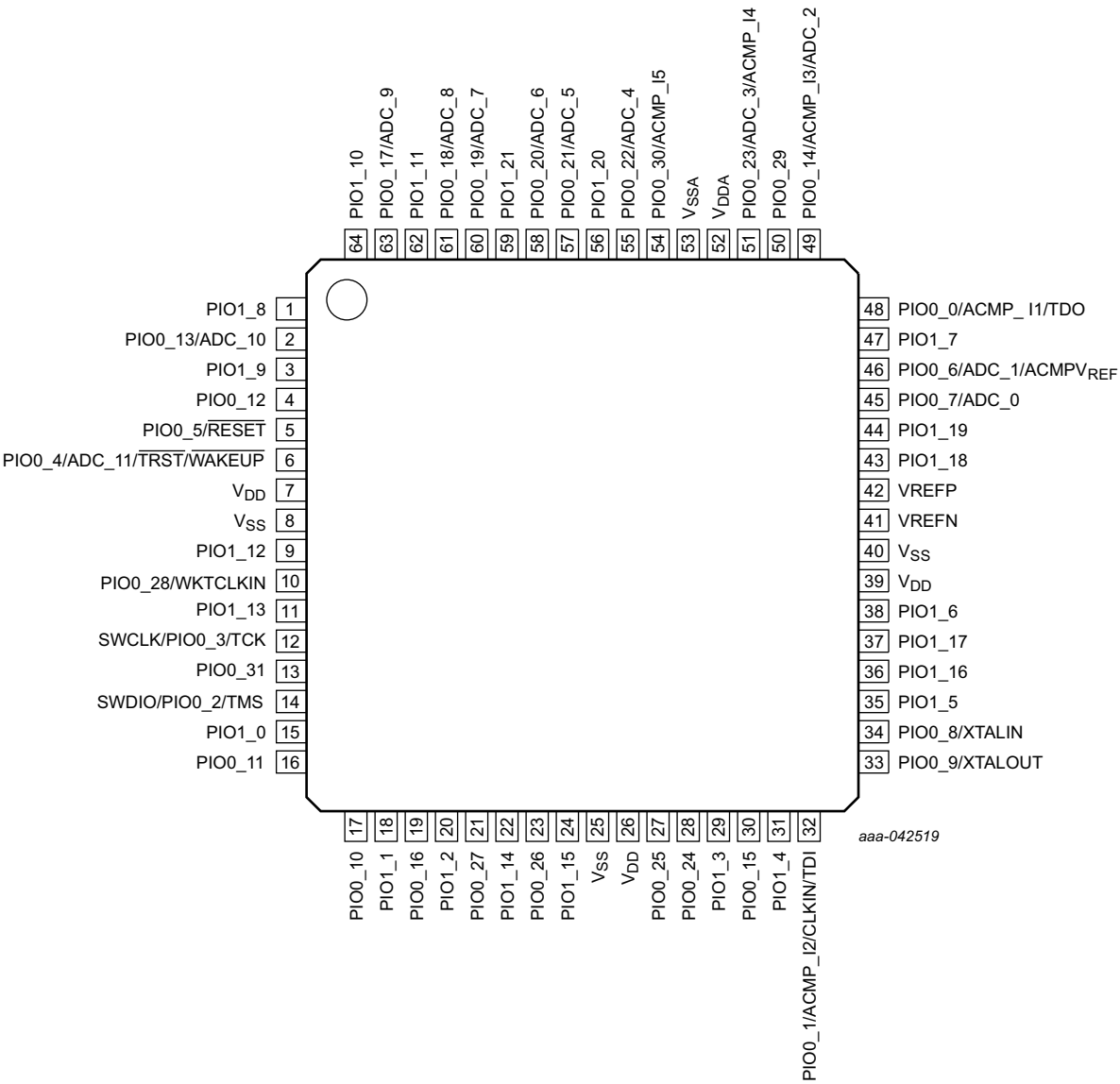
Fig 4. Pin configuration LQFP64 package
