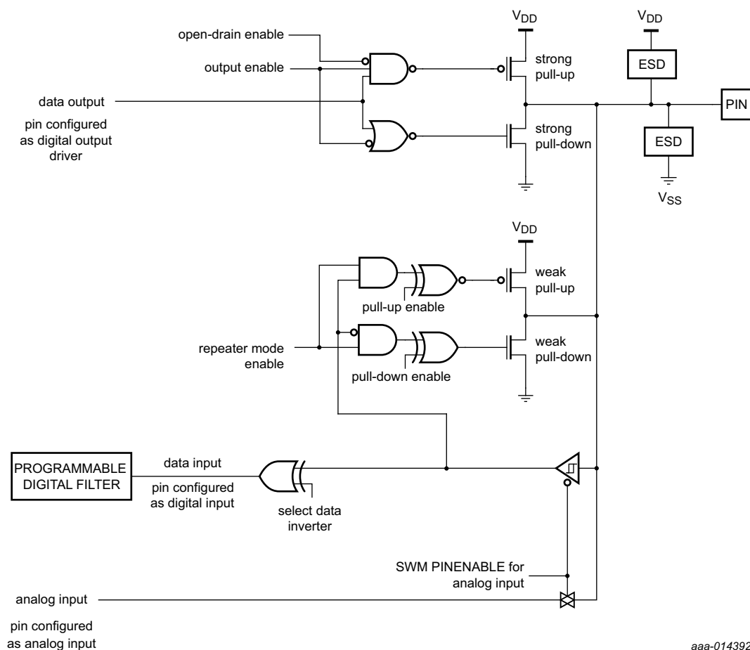
Fig 8. Standard I/O pad configuration
