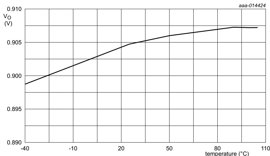
Fig 35. Typical internal voltage reference output voltage
