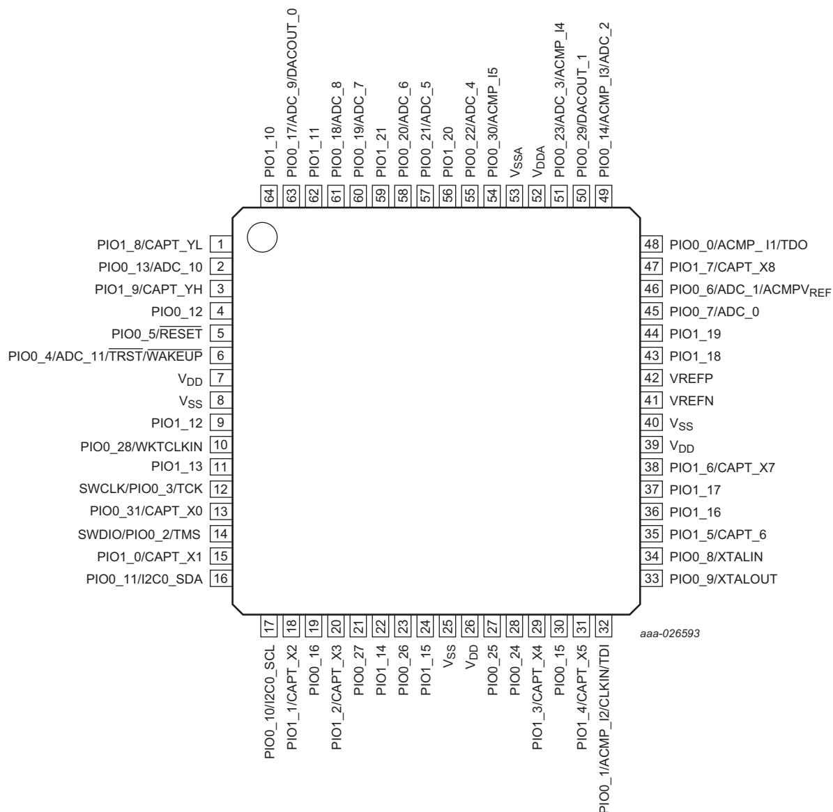
Fig 4. Pin configuration LQFP64 package
