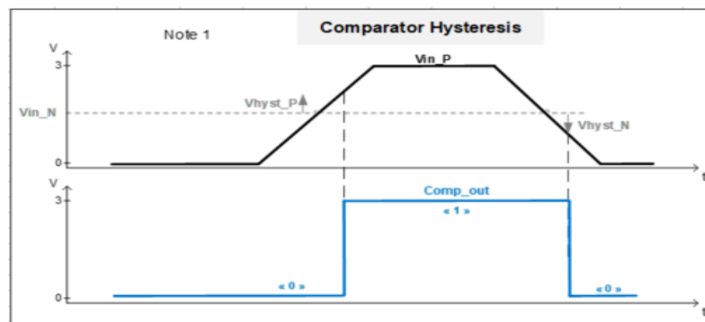
Fig 23. Comparator Hysteresis
