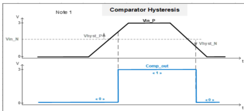
Fig 24. Comparator Hysteresis
