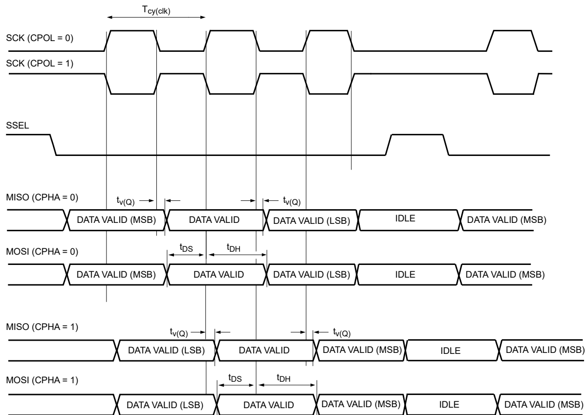
Figure 21. SPI slave timing
