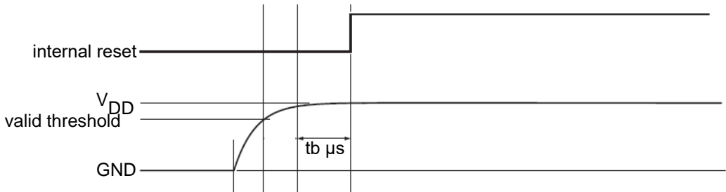
Figure 27. Start-up timing
