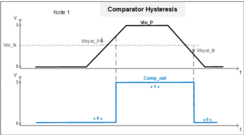
Figure 26. Comparator Hysteresis
