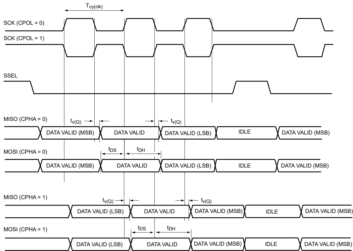
Figure 19. SPI slave timing
