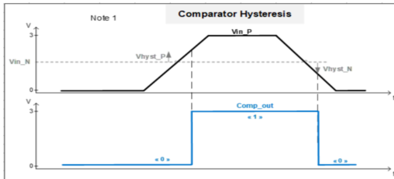
Fig 22. Comparator Hysteresis
