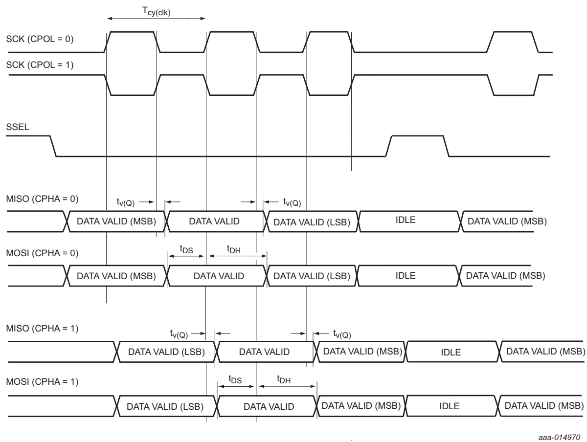
Fig 13. SPI slave timing
