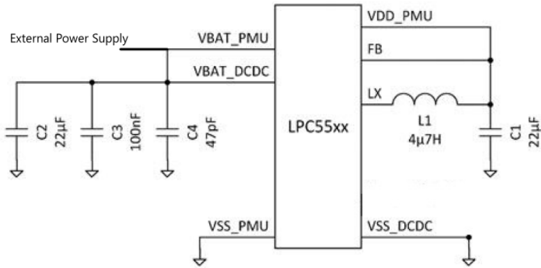
Fig 6. Using internal DC-DC converter
