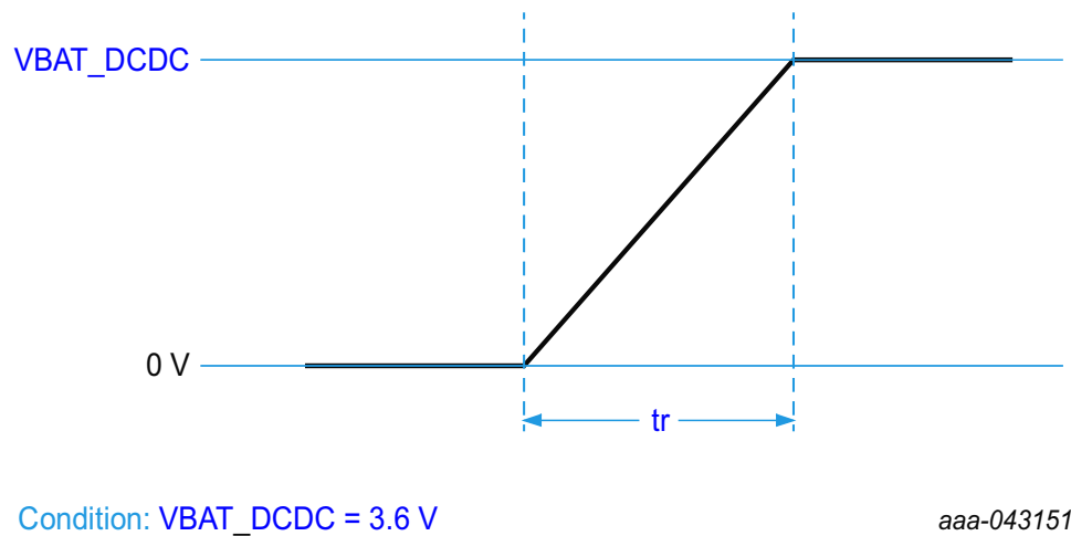
Fig 10. Power-up ramp
