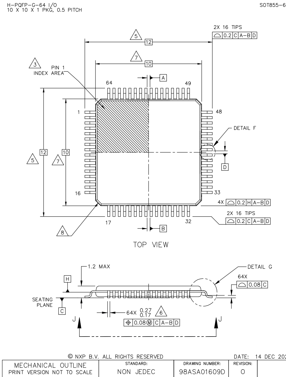
Fig 41. HTQFP64 Package outline 1
